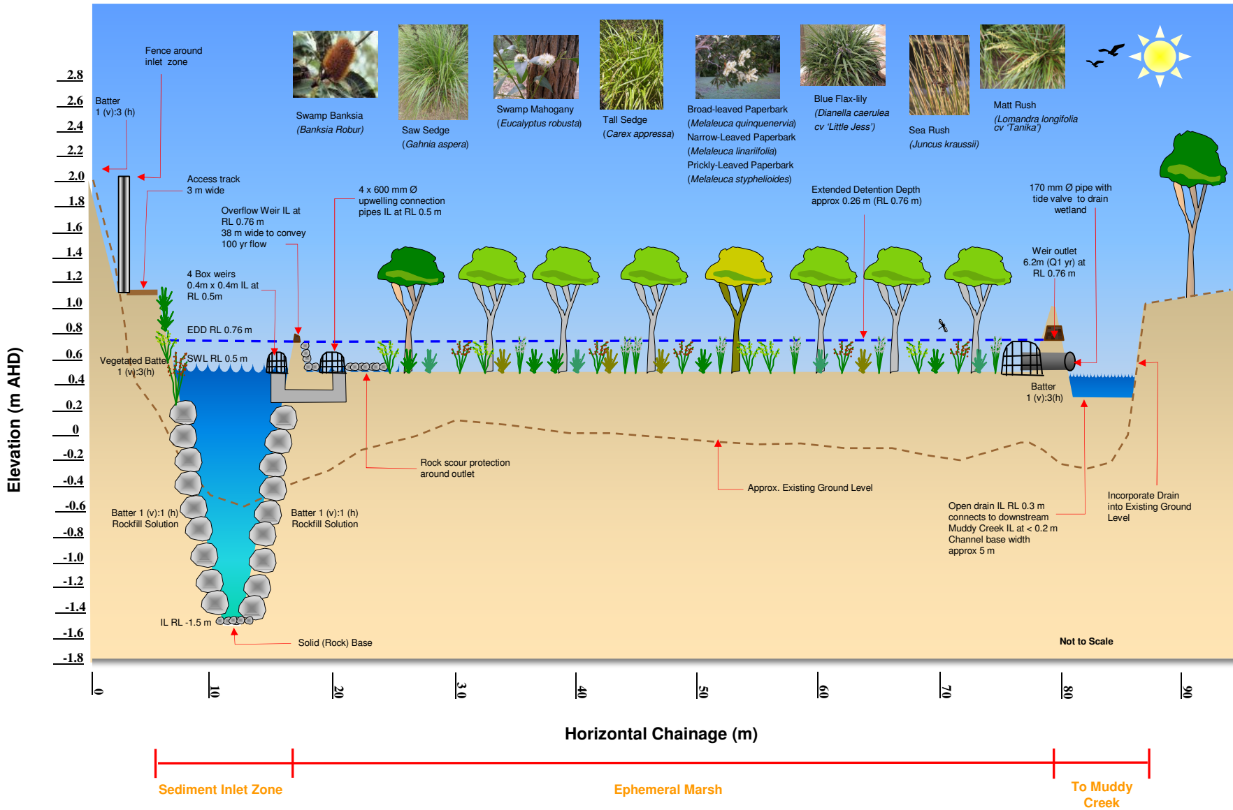
Sediment Basin Inlet Zone and Ephemeral Wetland Longitudinal Section A-A1
